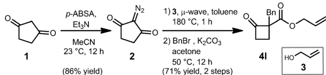
Scheme 1. Construction of allyl 1-benzyl-2-oxocyclobutane-carboxylate ( 4I ).
