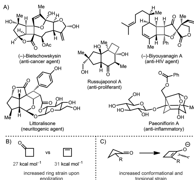
Figure 1. A) Representative bioactive natural products possessing cyclobutanoid core structures. B) Increased ring strain generated upon enolization. C) Increased conformational and torsional strain.
